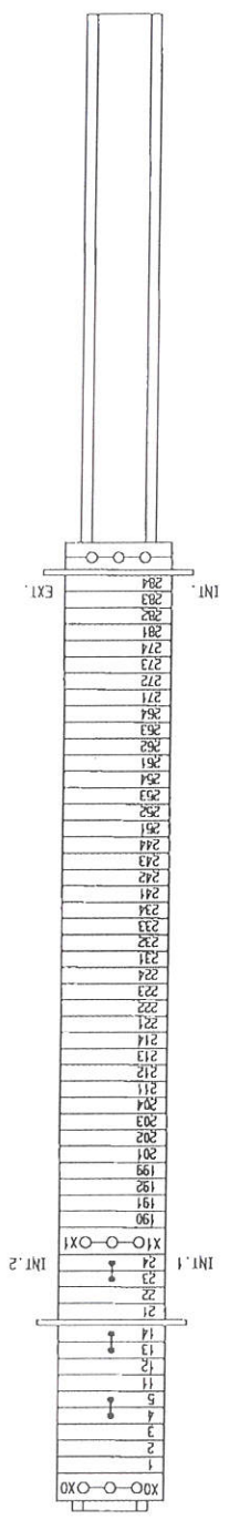
TERMINAL ARRANGEMENT (VERTICAL MOUNT.) (UPPER RAIL) PLINTARRANGEMANG (LODRAT MONT.) (DYRE SKENA)
